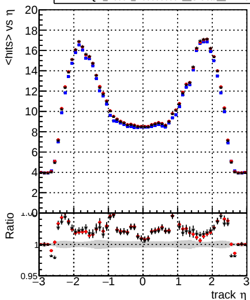
DQM_V0001_R000000001_Global_CKF_RECO DQM_V0001_R000000001_Global_mkFit1_RECO DQM_V0001_R000000001_Global_mkFit2_RECO
