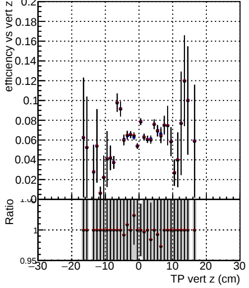
Efficiency vs vert z —●— DQM_V0001_R000000001_Global_CKF_RECO —●— DQM_V0001_R000000001_Global_mkFit1_RECO —●— DQM_V0001_R000000001_Global_mkFit2_RECO
