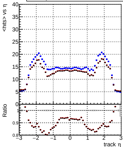
mean hits — DQM_V0001_R000000001_Global_CKF_RECO — DQM_V0001_R000000001_Global_mkFit1_RECO — DQM_V0001_R000000001_Global_mkFit2_RECO
