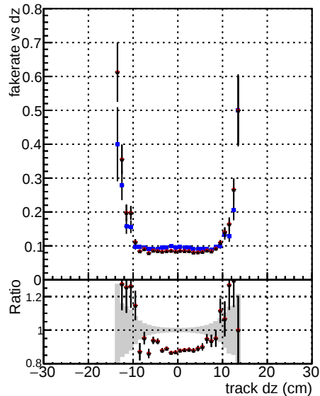
DOM V0001 R0000000001 Global CKF RECO Fake rate vs d Blue dots Red dots Black line Blue line Red line Blue dots Red dots Black line Blue line Red line
