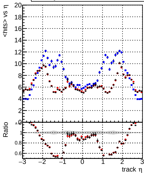
mean hits — DQM_V0001_R0000000001_Global_CKF_RECO — DQM_V0001_R0000000001_Global_mkFit1_RECO — DQM_V0001_R0000000001_Global_mkFit2_RECO
