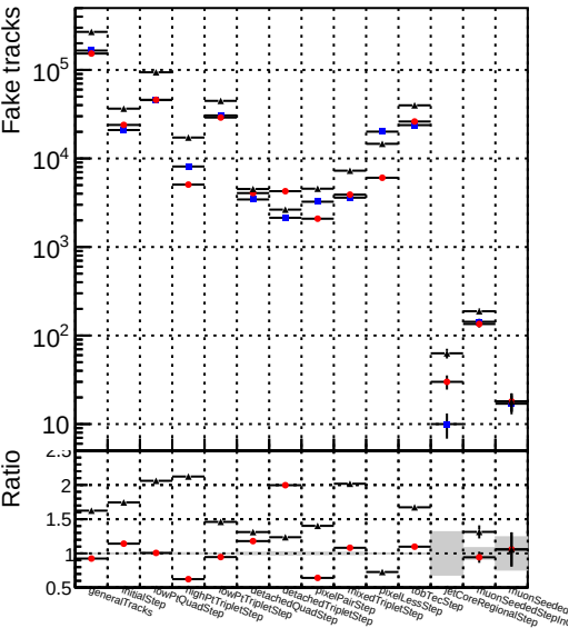
Numbe ● DQM_V0001_R0000000001_Global_mkFit1 RECO ★ DQM_V0001_R0000000001_Global_mkFit2 RECO
