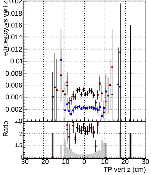
Efficiency vs. TP vert z (cm) Blue line with dots DQM_V0001_R000000001_Global_CKF_RECO Red line with dots DQM_V0001_R000000001_Global_mkFit1_RECO Black line with dots DQM_V0001_R000000001_Global_mkFit2_RECO
