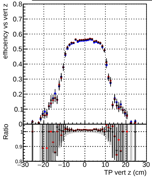
Efficiency vs vert z —●— DQM_V0001_R0000000001_Global_CKF_RECO —●— DQM_V0001_R0000000001_Global_mkFit1_RECO —●— DQM_V0001_R0000000001_Global_mkFit2_RECO
