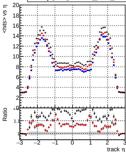
mean hit — DQM_V0001_R0000000001_Global_CKF_RECO — DQM_V0001_R0000000001_Global_mkFit1_RECO — DQM_V0001_R0000000001_Global_mkFit2_RECO
