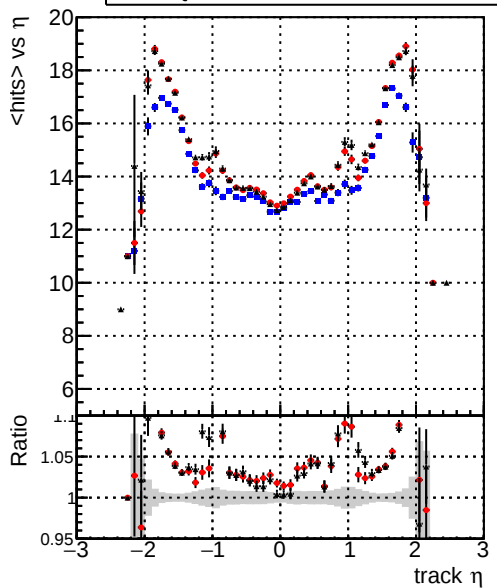
mean hits vs \eta — DQM_V0001_R0000000001_Global_CKF_RECO — DQM_V0001_R0000000001_Global_mkFit1_RECO — DQM_V0001_R0000000001_Global_mkFit2_RECO
