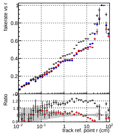
—●— DQM_V0001_R000000001 Global CKF RECO —●— DQM_V0001_R000000001 Global mkFit1 RECO —●— DQM_V0001_R000000001 Global mkFit2 RECO
