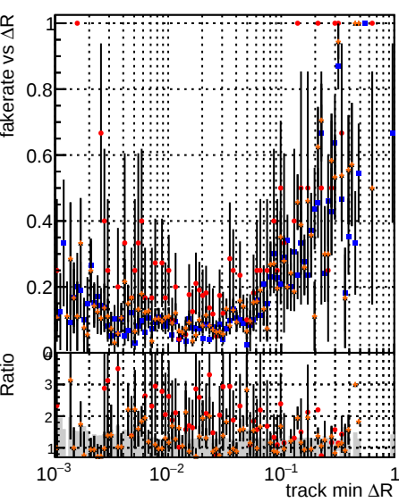
Fake rate vs \Delta R(\text{track, jet}) DOM CKE softQCD DOM mkrFit softQCD-ncp DOM mkrFit softQCD-newTr3
