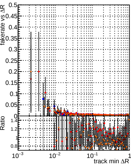
Fake rate vs \Delta R(\text{track, jet}) Legend: DOM CKE softQCD DOM-mkFit softQCD-ncp DOM-mkFit-softQCD-newTr3
