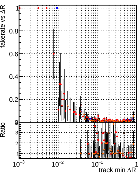
Fake rate vs ΔR(track, jet) Legend: DOM (black) CKE (blue) softQCD (red) ncp (orange) newTr3 (grey)
