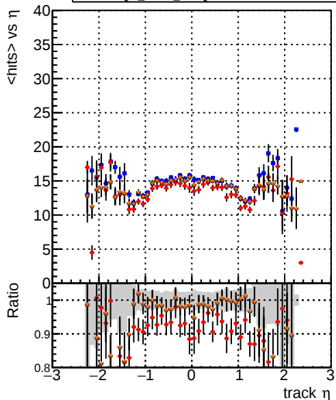
Legend: DQM_CKF_softQCD (blue), DQM_mkFit_softQCD (red), DQM_mkFit_softQCD-ncp (black), DQM_mkFit_softQCD-newTr3 (orange) mean hits
