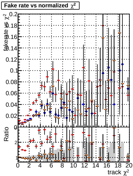
Fake rate vs. Legend: DOM, GKE, softOCB, OCB
