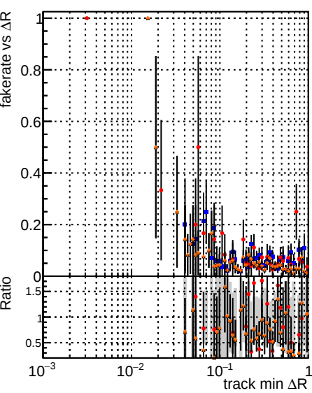
Fake rate vs ΔR(track, jet) DOM CKE softQCD DOM mkrFit softQCD-ncp DOM mkrFit softQCD-newTr3
