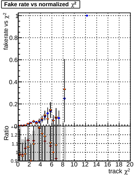
Fake rate vs. Legend: DQM, SKF, softOCB, OCB
