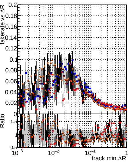
Fake rate vs ΔR(track, jet) Legend: DOM CKE softQCD mkrFit softQCD-ncp softQCD-newTr3
