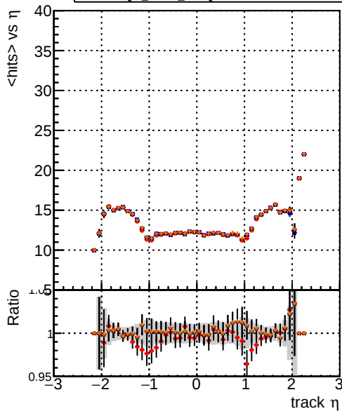
mean hit DOM_CKF_softQCD DOM_mkFit_softQCD DOM_mkFit_softQCD-ncp DOM_mkFit_softQCD-newTr3
