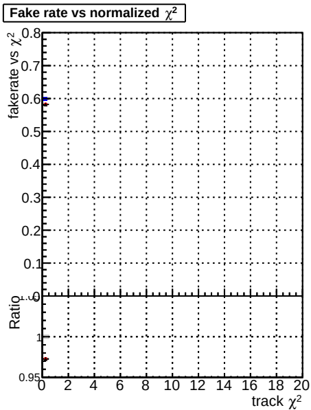
Fake rate vs. \chi^2 Legend: DOM CKF softOCB DOM CKF softOCB-newTr2 DOM CKF softOCB-newTr2
