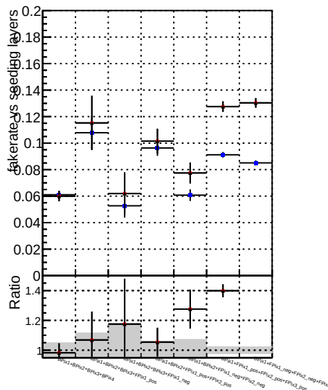
Fake rate vs. DOM CKF softOCB DOM CKF softOCB-newTr2
