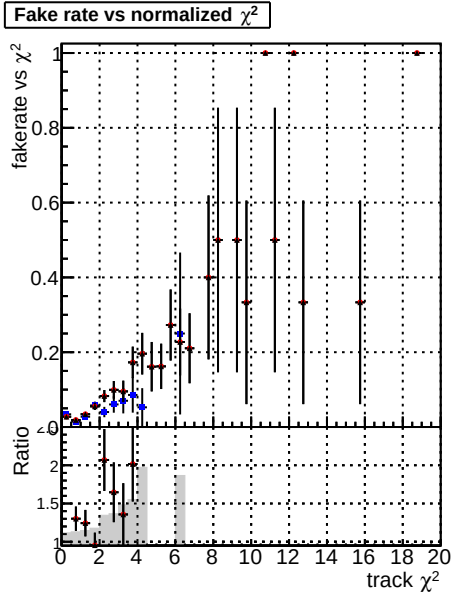
Fake rate vs. DOM CKF softQCB DOM mktFit softQCB-newTr2
