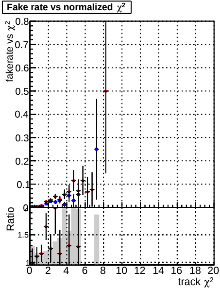
Fake rate vs. \chi^2 Legend: DOM (blue), CKF (red), softOCB (grey), BQM (black), mktFit (green), softOCB-newTr2 (purple)
