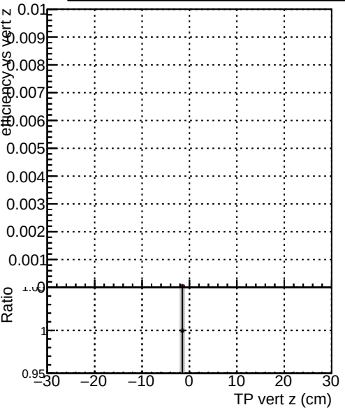
Efficiency vs vert z Legend: DQM_CKF_softQCD (blue line with dots) DQM_mkFit_softQCD (red line with dots) DQM_mkFit_softQCD-newTr2 (black line with dots)
