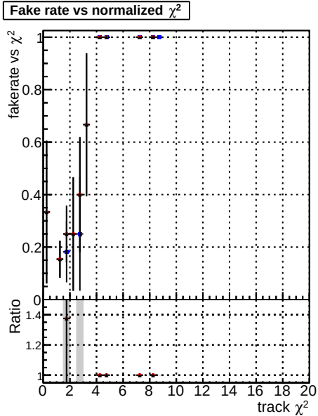
Fake rate vs. DOM CKF softOCB DOM mktFit softOCB-newTr2
