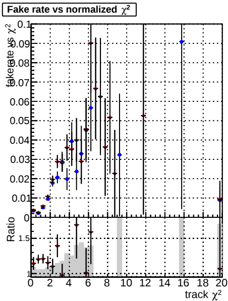
Fake rate vs. DOM CKF softQCD DOM CKF softQCD-newTr2
