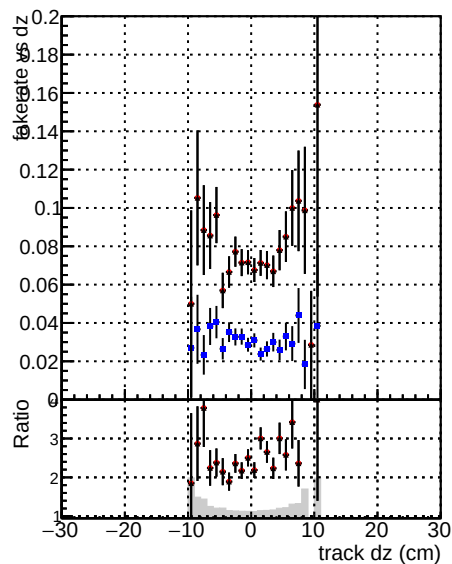
—•— DOM CKF softQCB —•— BOM mktFit softQCB-newTr2
