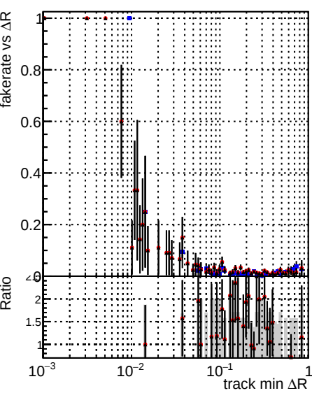
Legend: DOM_CKF_softQCD (black line with blue dots), DOM_mkFit_softQCD (black line with red dots), DOM_mkFit_softQCD-newTr2 (black line with black dots)
