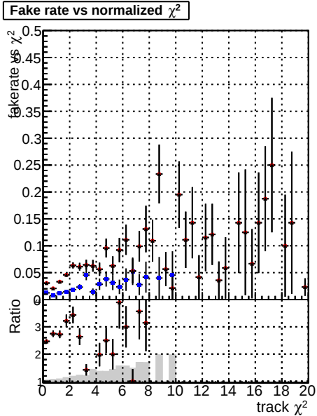
Fake rate vs. Legend: DOM, CKF, softOCB, BOM, mkt, softOCB-newTr
