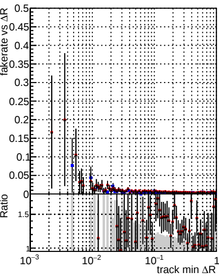
Fake rate vs ΔR(track, jet) Legend: DOM_CKF_softQCD (black line with blue dots) DOM_mkFit_softQCD (red line with red dots) DOM_mkFit_softQCD-newTr (black line with black dots)
