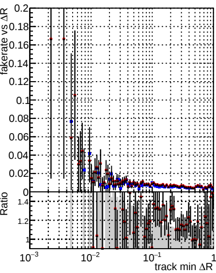
Legend: DQM_CKF_softQCD (black line with blue dots), DQM_mkFit_softQCD (red line with red dots), DQM_mkFit_softQCD-newTr (black line with black dots)
