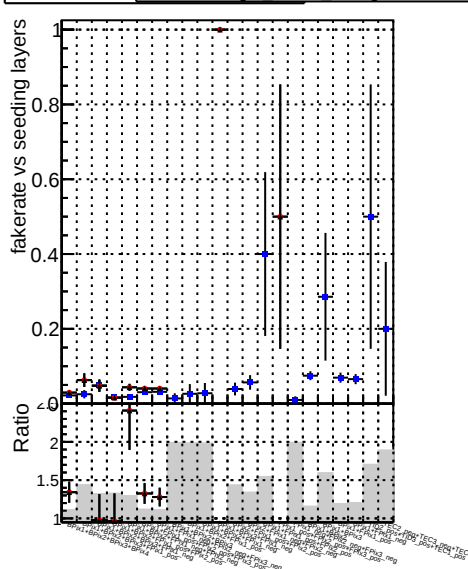
Fake rate vs. DOM CKF softOCB BOM mktFit softOCB-newTr
