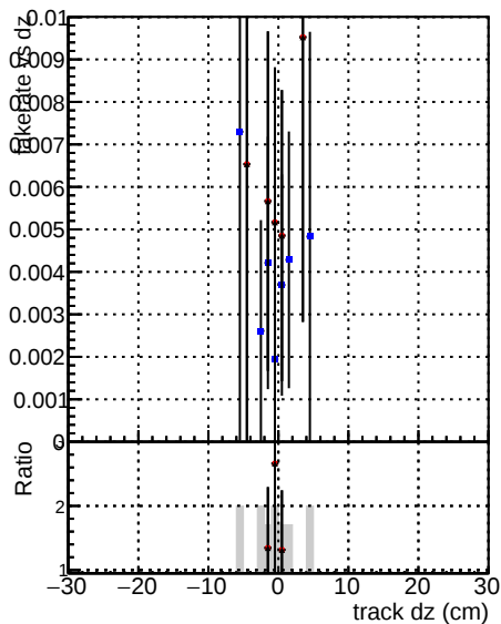
DOM CKF softQCB DOM-mkFit softQCB-newTr
