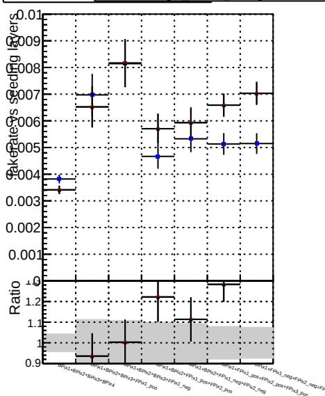
Fake rate vs. DOM CKF softOCB DOM mktFit softOCB-newTr
