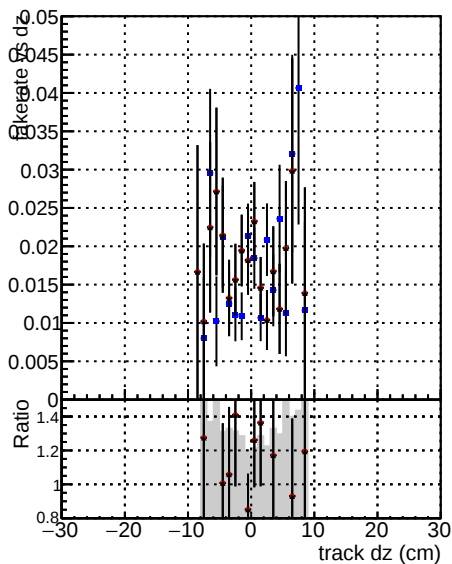
Fake rate vs dz DOM CKE softQCB DOM mktFit softQCB DOM mktFit softQCB-newTr
