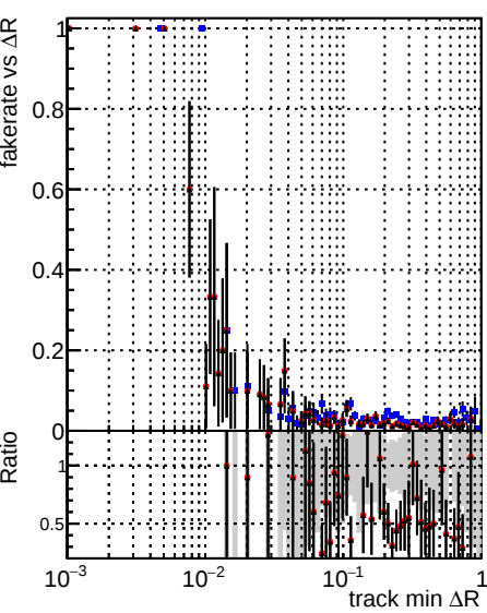
Legend: DOM_CKF_softQCD (blue line with dots), DOM_mkFit_softQCD (red line with dots), DOM_mkFit_softQCD-newTr (black line with dots)
