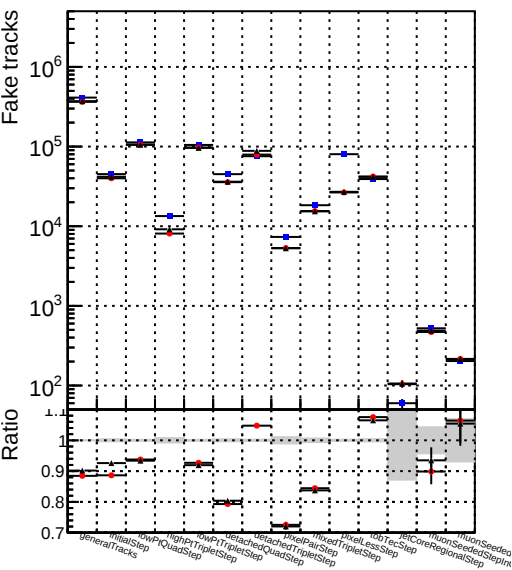
Number ● DQM_mkFit_TTbarPU-noDNN3 ★ DQM_mkFit_TTbarPU-clonerfix3
