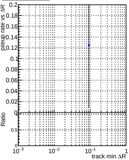
Legend: DQM_CKF_TTbarPU (black), DQM_mkFit_TTbarPU-noDNN3 (red), DQM_mkFit_TTbarPU-clonerfix3 (blue)
