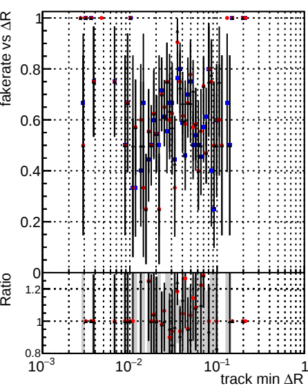
Legend: DQM_CKF_TTbarPU (black), DQM_mkFit_TTbarPU-noDNN3 (red), DQM_mkFit_TTbarPU-clonerfix3 (blue)
