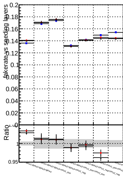
Fake rate vs. DOM CKF T\bar{T} barPU DOM mkt T\bar{T} barPU-noDNN3 DOM mkt T\bar{T} barPU-clonerfix3
