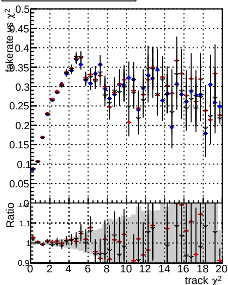
Fake rate vs. DOM CKF T\bar{T} barPU DOM mkt T\bar{T} barPU-noDNN3 DOM mkt T\bar{T} barPU-clonerfix3
