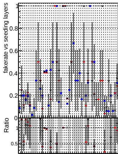
Fake rate vs. — DOM CKF TTbarPU — DOM CKF TTbarPU-noDNN3 — DOM mktFit TTbarPU-clonerfix3
