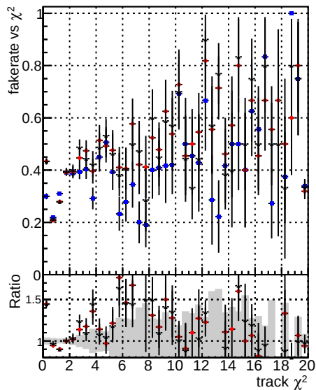
Fake rate vs. — DOM CKF TTbarPU — DOM CKF TTbarPU-noDNN3 — DOM mktFit TTbarPU-clonerfix3
