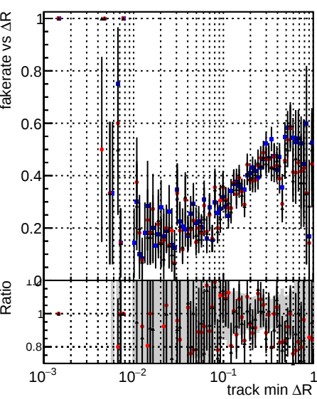
Fake rate vs \Delta R(\text{track, jet}) DQM_CKF_TTbarPU DQM_mkFit_TTbarPU-noDNN3 DQM_mkFit_TTbarPU-clonerfix3
