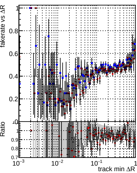
Legend: DQM_CKF_TTbarPU (blue stars), DQM_mkFit_TTbarPU-noDNN3 (red stars), DQM_mkFit_TTbarPU-clonerfix3 (black stars)
