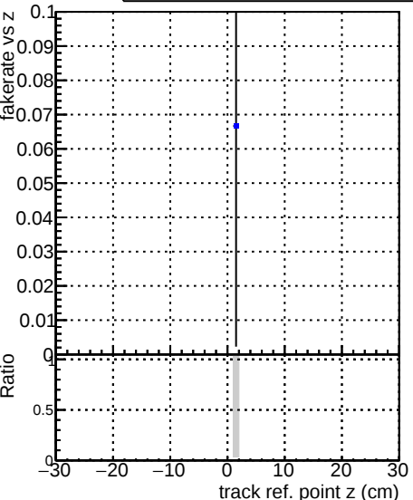
Fake rate vs verpos DQM_CKF_TTbarPU DQM_mkFit_TTbarPU-noDNN3 DQM_mkFit_TTbarPU-clonerfix3
