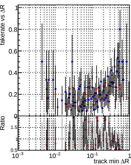
Legend: DQM_CKF_TTbarPU (blue dots), DQM_mkFit_TTbarPU-noDNN3 (red dots), DQM_mkFit_TTbarPU-clonerfix3 (black dots)
