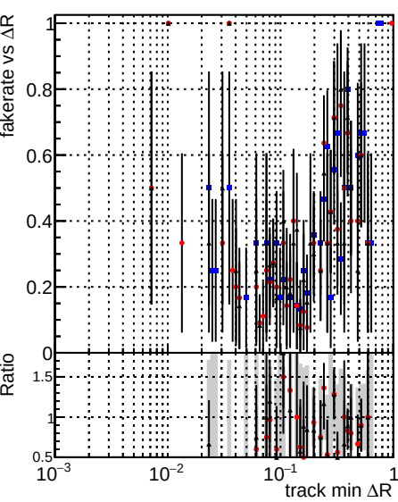
DOM_CKF_TTbarPU DOM_mkFit_TTbarPU-noDNN3 DOM_mkFit_TTbarPU-clonerfix3
