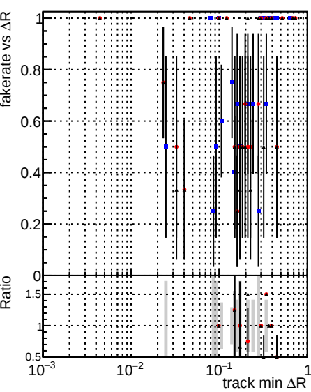
Fake rate vs \Delta R (track, jet) DQM_CKF_TTbarPU DQM_mkFit_TTbarPU-noDNN3 DQM_mkFit_TTbarPU-clonerfix3
