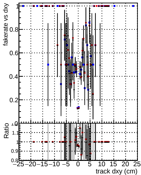
Legend for Fake rate vs dxy: DOM CKE TTbarPU (blue dots) DOM mktFit TTbarPU-noDNN3 (red dots) DOM mktFit TTbarPU-clonerfix3 (black dots)
