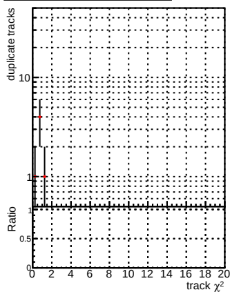
N of duplicate tracks vs. \chi^2
