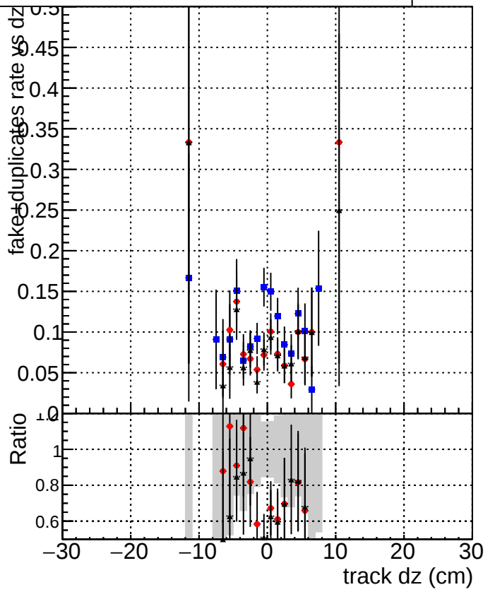
Legend: ■ DQM_CKF_TTbarPU ● DQM_mkFit_TTbarPU-noDNN3 ▲ DQM_mkFit_TTbarPU-clonerfix3
